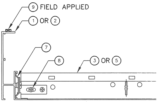
GRID TO TRIM CONNECTION
